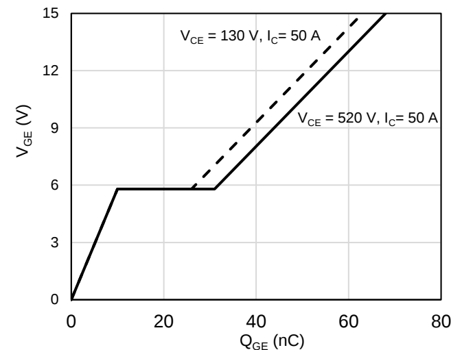
Figure 16: Gate-Charge Characteristics
